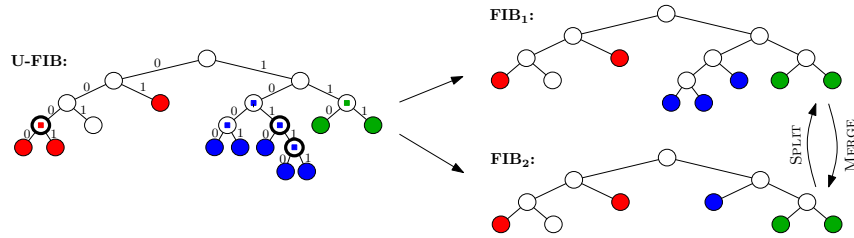
Fig. 2. One-bit tries representing a U-FIB and two possible compressions to the FIBs. Mergeable nodes are marked with small squares in the center. Nodes consolidated for the creation of FIB 1 are drawn with bold lines.
